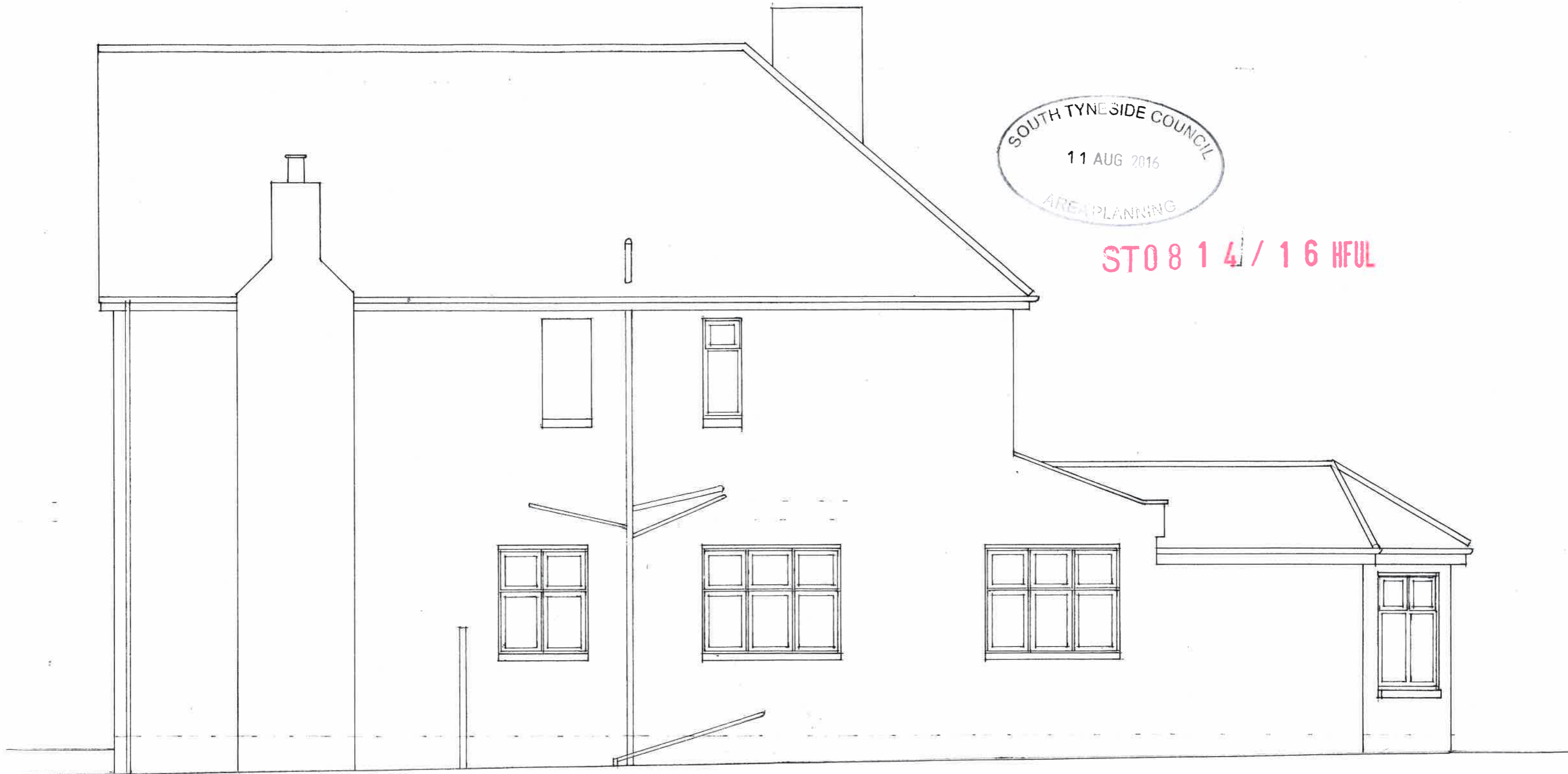
WEST ELEVATION
